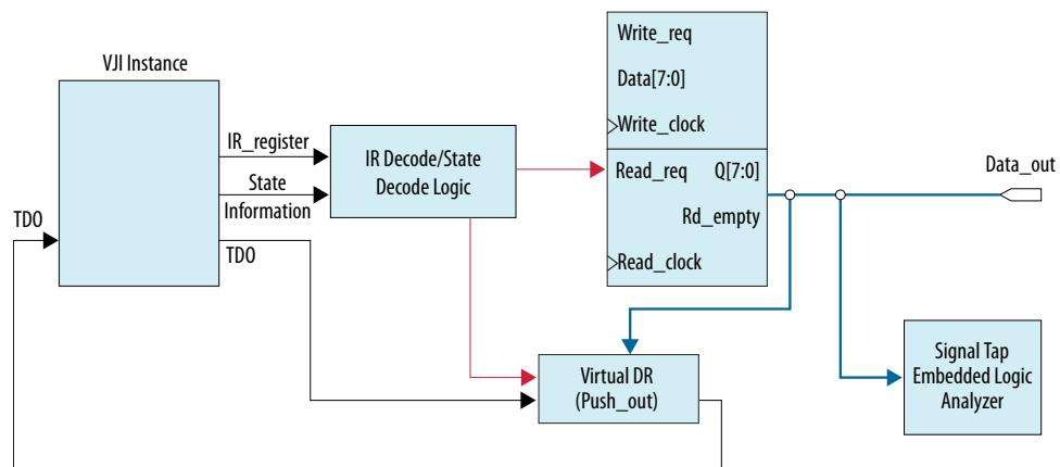
Figure 22. Read Side Logic for DCFIFO Design Example
