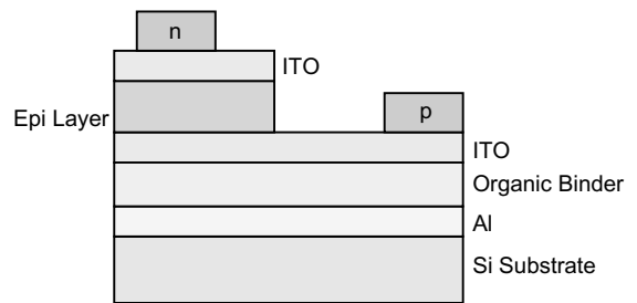
Figure 11. OMA-Chip
