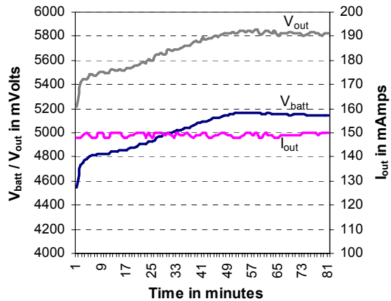
Figure 6. NiMH Charging Profile
